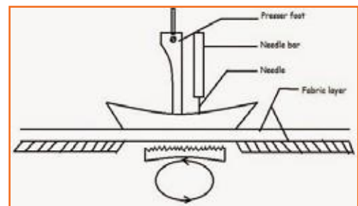
Fig.2.1.14: Drop Feed Mechanism
