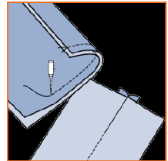
Fig.2.2.6: Superimposed Seams
